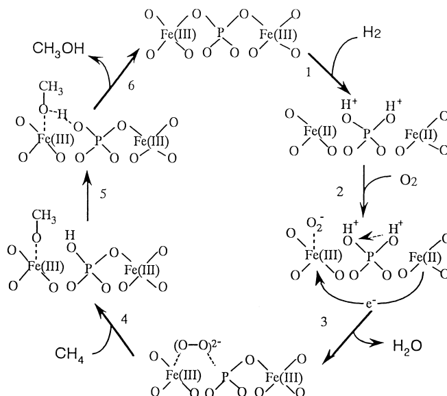
Scheme 1. Proposed catalytic cycle for the conversion of \text{CH}_4 to \text{CH}_3\text{OH} [18].
