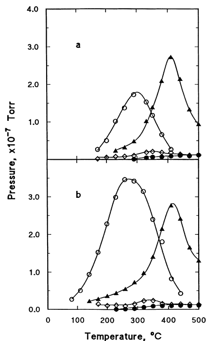
Fig. 3. Temperature-programmed surface reaction results after reaction of 3 mTorr CH_3\cdot radicals with 5.1% V_2O_5/SiO_2 for 30 min at 150°C followed by cooling to 50°C: (a) sample heated in vacuo; (b) sample heated in 7 mTorr H_2O : (○) CH_3OH , (▲) HCHO, (◇) CO, (●) CO_2 [24].
